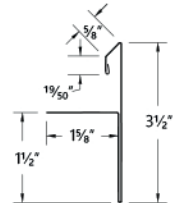
50 ABS Slim Line Rake (ABSSLRcc)
