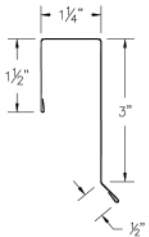
45 ABS Rake Trim (ABSRtcc)
