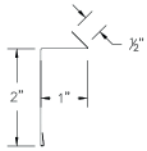
43 ABS Counter Flashing (ABSCFcc)
