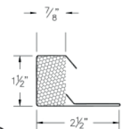
12 ABS Vented "Z" Closure (ABSZVcc)
