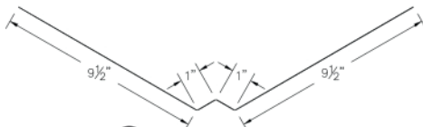
19 ABS W Valley (ABS WVcc)
